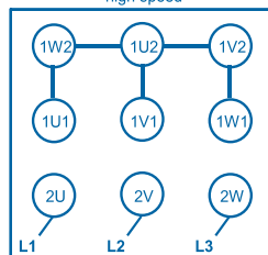
YY connection
