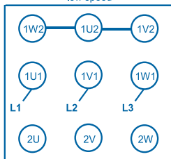
low speed
