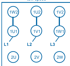
Δ connection
