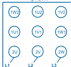
high speed
