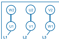
Δ connection
