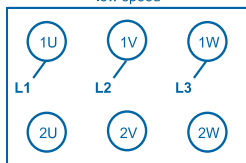
low speed
